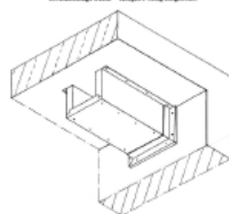
WAS 3-seitig, Kanal Direktmontage Decke
